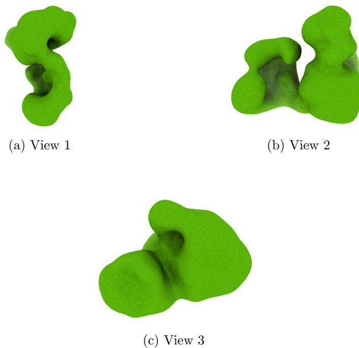
Figure 4: Isosurface at threshold=4.250000. Views generated by ChimeraX at a the following X, Y, Z angles: View 1 (0, -90, -90), View 2 (-90, 0, -90), View 3 (0, 0, 0).
