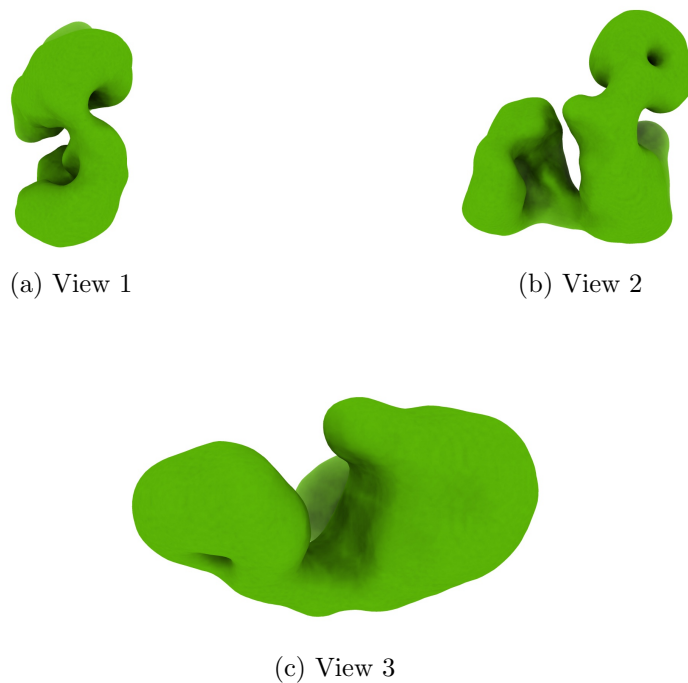
Figure 4: Isosurface at threshold=3.750000. Views generated by ChimeraX at a the following X, Y, Z angles: View 1 (0, -90, -90), View 2 (-90, 0, -90), View 3 (0, 0, 0).
