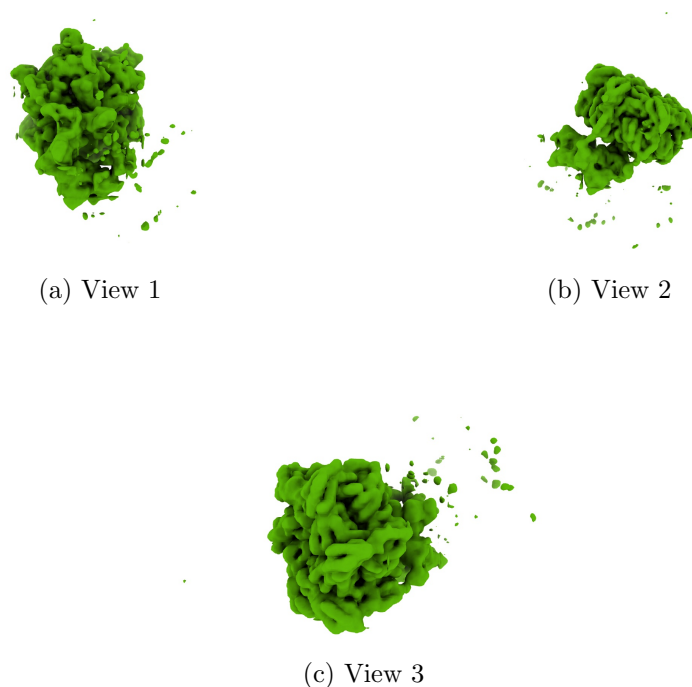
Figure 4: Isosurface at threshold=0.008300. Views generated by ChimeraX at a the following X, Y, Z angles: View 1 (0, -90, -90), View 2 (-90, 0, -90), View 3 (0, 0, 0).
