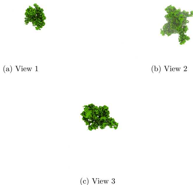
Figure 4: Isosurface at threshold=0.008860. Views generated by ChimeraX at a the following X, Y, Z angles: View 1 (0, -90, -90), View 2 (-90, 0, -90), View 3 (0, 0, 0).
