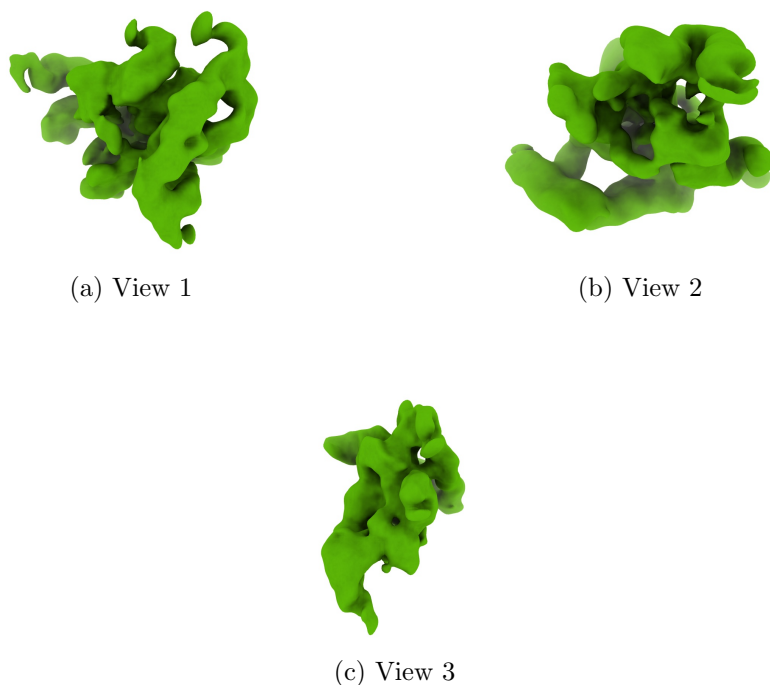
Figure 4: Isosurface at threshold=0.730000. Views generated by ChimeraX at a the following X, Y, Z angles: View 1 (0, -90, -90), View 2 (-90, 0, -90), View 3 (0, 0, 0).
