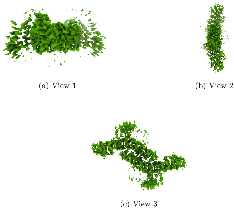
Figure 4: Isosurface at threshold=0.431000. Views generated by ChimeraX at a the following X, Y, Z angles: View 1 (0, -90, -90), View 2 (-90, 0, -90), View 3 (0, 0, 0).
