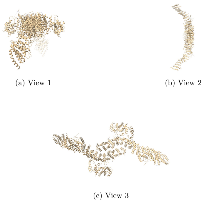
Figure 12: Input atomic model Views generated by ChimeraX at the following X, Y, Z angles: View 1 (0, -90, -90), View 2 (-90, 0, -90), View 3 (0, 0, 0).
