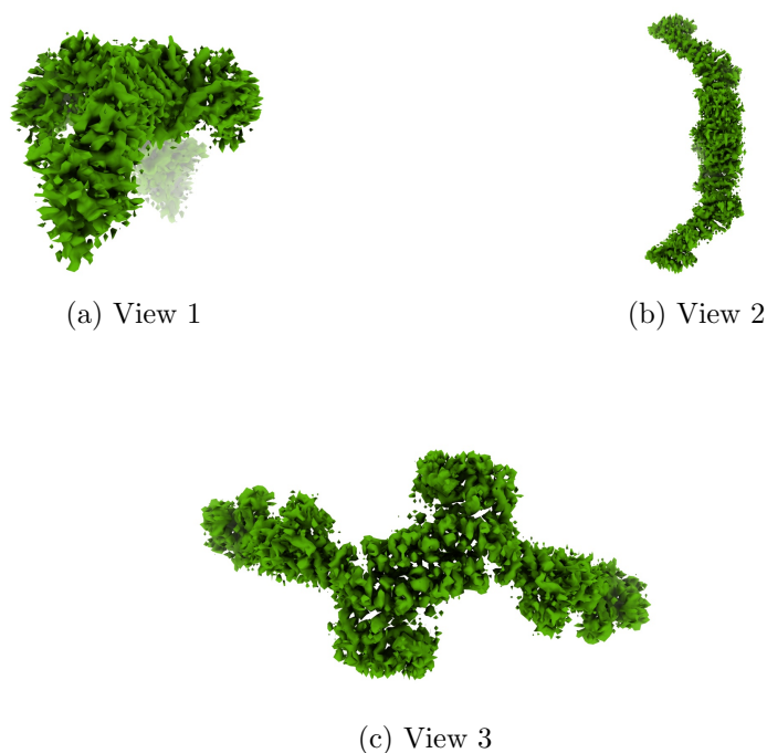
Figure 4: Isosurface at threshold=5.850000. Views generated by ChimeraX at a the following X, Y, Z angles: View 1 (0, -90, -90), View 2 (-90, 0, -90), View 3 (0, 0, 0).
