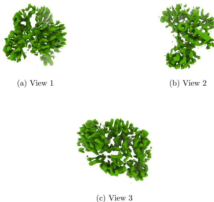
Figure 4: Isosurface at threshold=0.690000. Views generated by ChimeraX at a the following X, Y, Z angles: View 1 (0, -90, -90), View 2 (-90, 0, -90), View 3 (0, 0, 0).
