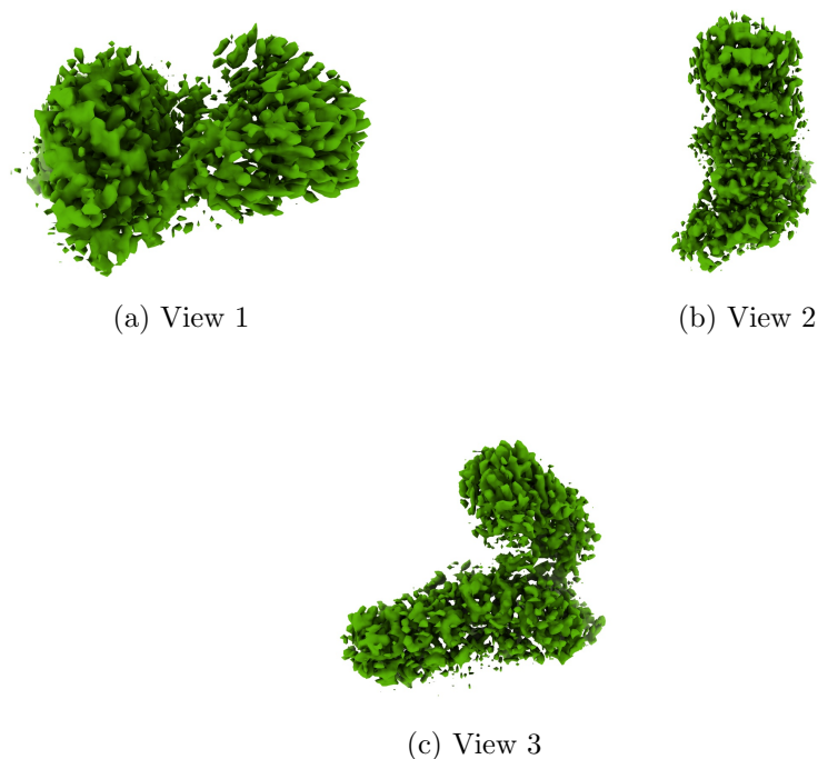
Figure 4: Isosurface at threshold=0.266000. Views generated by ChimeraX at a the following X, Y, Z angles: View 1 (0, -90, -90), View 2 (-90, 0, -90), View 3 (0, 0, 0).
