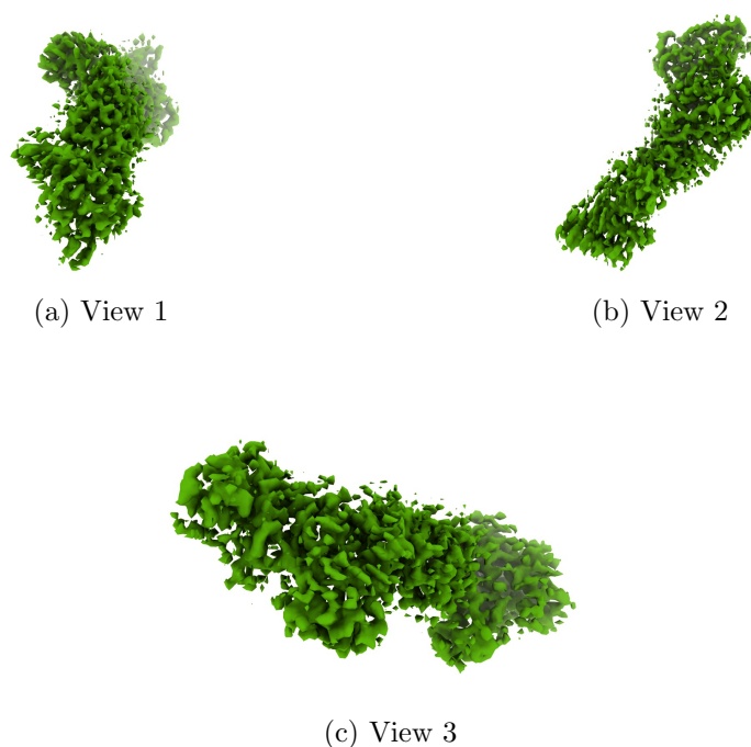
Figure 4: Isosurface at threshold=0.342000. Views generated by ChimeraX at a the following X, Y, Z angles: View 1 (0, -90, -90), View 2 (-90, 0, -90), View 3 (0, 0, 0).
