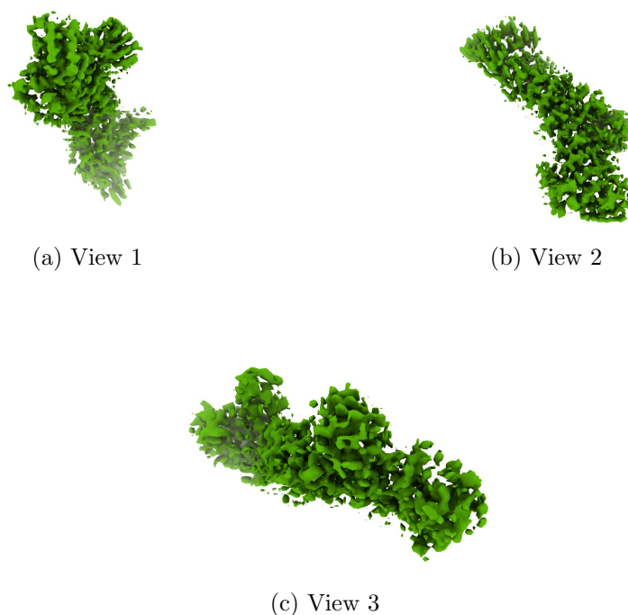
Figure 4: Isosurface at threshold=0.317000. Views generated by ChimeraX at a the following X, Y, Z angles: View 1 (0, -90, -90), View 2 (-90, 0, -90), View 3 (0, 0, 0).
