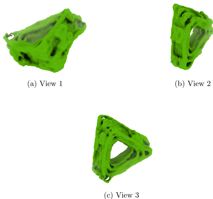
Figure 4: Isosurface at threshold=0.024400. Views generated by ChimeraX at a the following X, Y, Z angles: View 1 (0, -90, -90), View 2 (-90, 0, -90), View 3 (0, 0, 0).
