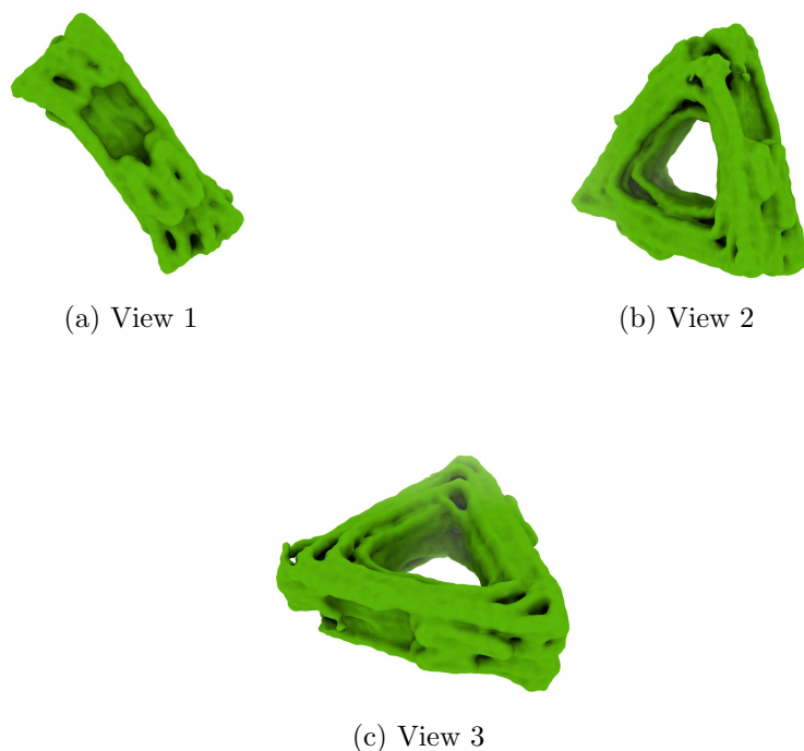
Figure 4: Isosurface at threshold=0.019400. Views generated by ChimeraX at a the following X, Y, Z angles: View 1 (0, -90, -90), View 2 (-90, 0, -90), View 3 (0, 0, 0).
