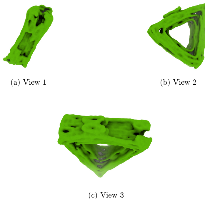
Figure 4: Isosurface at threshold=0.034500. Views generated by ChimeraX at a the following X, Y, Z angles: View 1 (0, -90, -90), View 2 (-90, 0, -90), View 3 (0, 0, 0).
