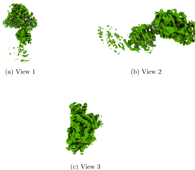
Figure 4: Isosurface at threshold=8.000000. Views generated by ChimeraX at a the following X, Y, Z angles: View 1 (0, -90, -90), View 2 (-90, 0, -90), View 3 (0, 0, 0).
