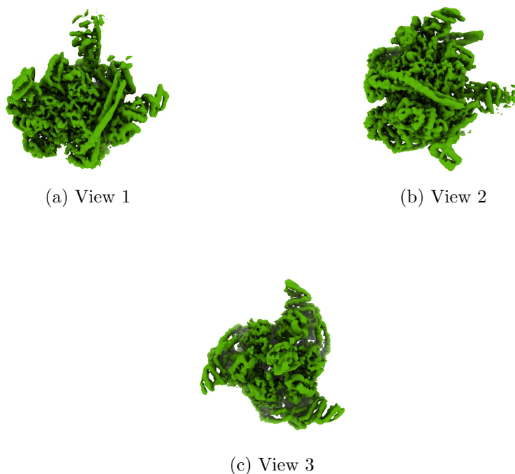
Figure 4: Isosurface at threshold=0.735000. Views generated by ChimeraX at a the following X, Y, Z angles: View 1 (0, -90, -90), View 2 (-90, 0, -90), View 3 (0, 0, 0).
