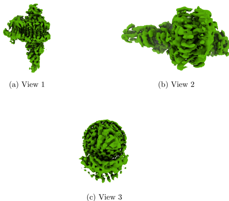
Figure 4: Isosurface at threshold=0.442000. Views generated by ChimeraX at a the following X, Y, Z angles: View 1 (0, -90, -90), View 2 (-90, 0, -90), View 3 (0, 0, 0).
