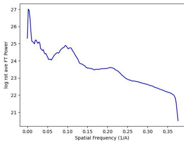
Figure 35: Logarithm of the radial average of the input map power in Fourier space.
