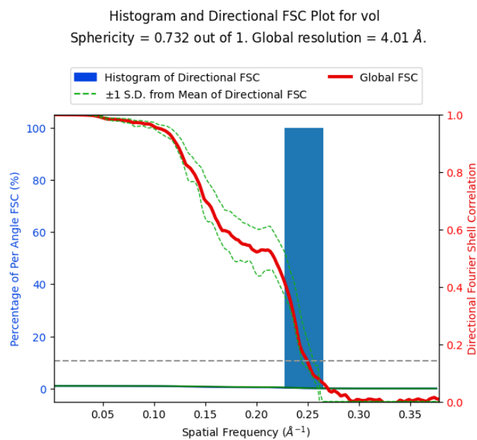
Figure 34: Global FSC and histogram of the directional FSC.
