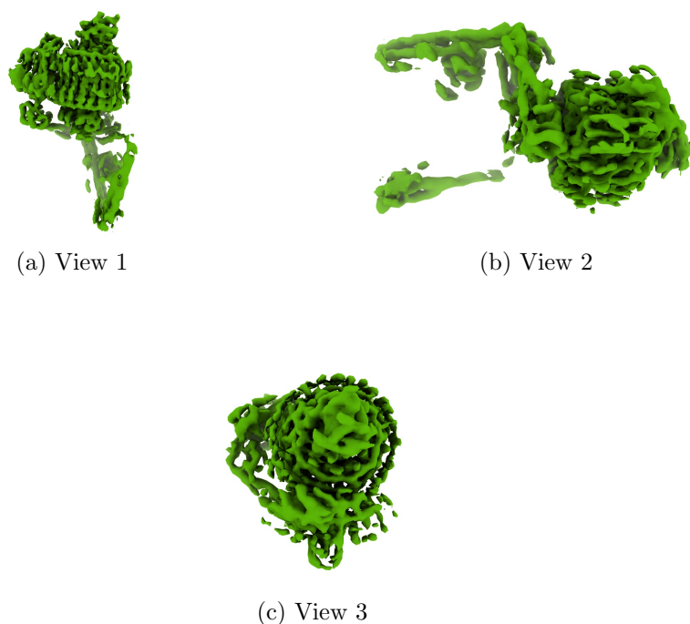
Figure 4: Isosurface at threshold=0.640000. Views generated by ChimeraX at a the following X, Y, Z angles: View 1 (0, -90, -90), View 2 (-90, 0, -90), View 3 (0, 0, 0).
