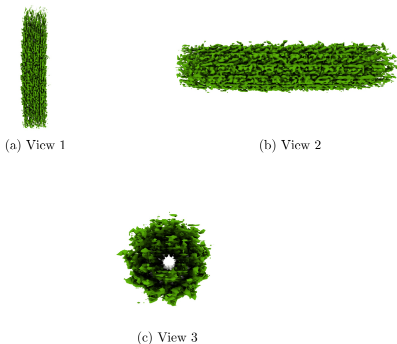
Figure 4: Isosurface at threshold=0.218000. Views generated by ChimeraX at a the following X, Y, Z angles: View 1 (0, -90, -90), View 2 (-90, 0, -90), View 3 (0, 0, 0).
