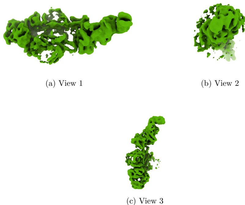
Figure 4: Isosurface at threshold=0.016800. Views generated by ChimeraX at a the following X, Y, Z angles: View 1 (0, -90, -90), View 2 (-90, 0, -90), View 3 (0, 0, 0).
