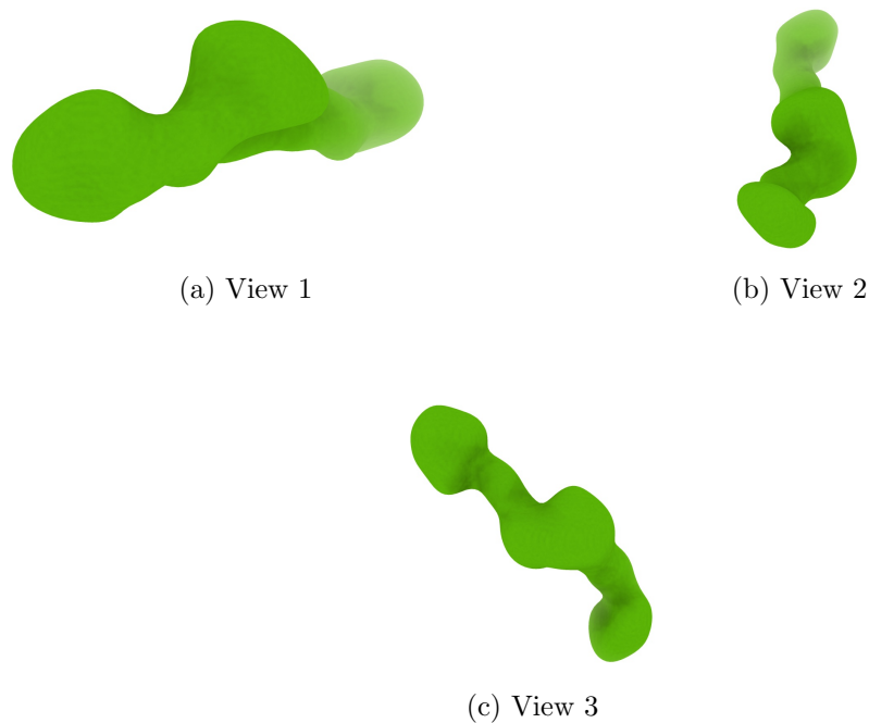
Figure 4: Isosurface at threshold=0.986000. Views generated by ChimeraX at a the following X, Y, Z angles: View 1 (0, -90, -90), View 2 (-90, 0, -90), View 3 (0, 0, 0).
