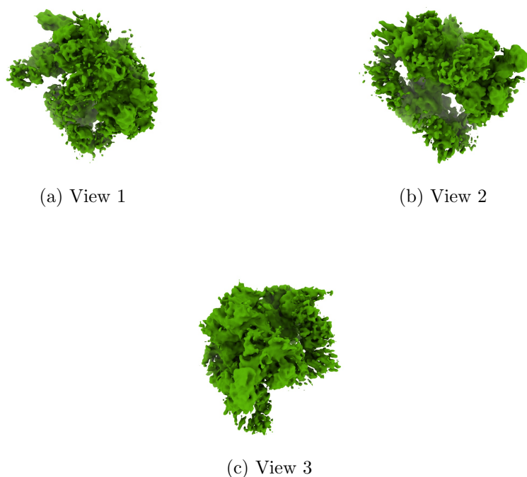
Figure 4: Isosurface at threshold=0.037000. Views generated by ChimeraX at a the following X, Y, Z angles: View 1 (0, -90, -90), View 2 (-90, 0, -90), View 3 (0, 0, 0).
