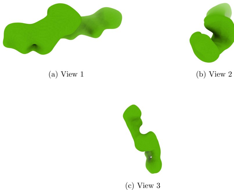
Figure 4: Isosurface at threshold=0.975000. Views generated by ChimeraX at a the following X, Y, Z angles: View 1 (0, -90, -90), View 2 (-90, 0, -90), View 3 (0, 0, 0).
