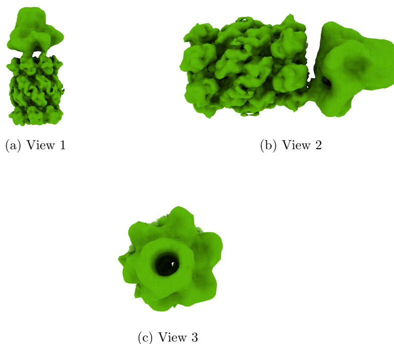
Figure 4: Isosurface at threshold=3.200000. Views generated by ChimeraX at a the following X, Y, Z angles: View 1 (0, -90, -90), View 2 (-90, 0, -90), View 3 (0, 0, 0).
