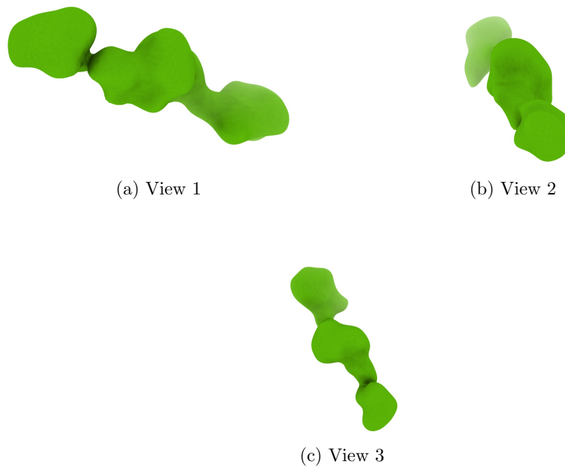
Figure 4: Isosurface at threshold=0.897000. Views generated by ChimeraX at a the following X, Y, Z angles: View 1 (0, -90, -90), View 2 (-90, 0, -90), View 3 (0, 0, 0).
