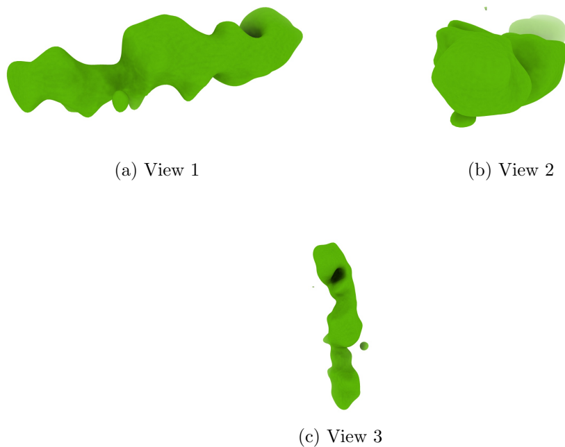
Figure 4: Isosurface at threshold=0.768000. Views generated by ChimeraX at a the following X, Y, Z angles: View 1 (0, -90, -90), View 2 (-90, 0, -90), View 3 (0, 0, 0).
