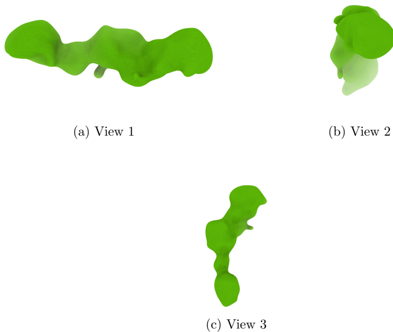
Figure 4: Isosurface at threshold=0.696000. Views generated by ChimeraX at a the following X, Y, Z angles: View 1 (0, -90, -90), View 2 (-90, 0, -90), View 3 (0, 0, 0).
