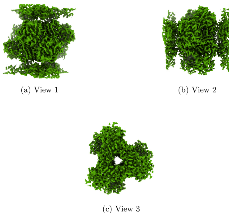
Figure 4: Isosurface at threshold=1.250000. Views generated by ChimeraX at a the following X, Y, Z angles: View 1 (0, -90, -90), View 2 (-90, 0, -90), View 3 (0, 0, 0).
