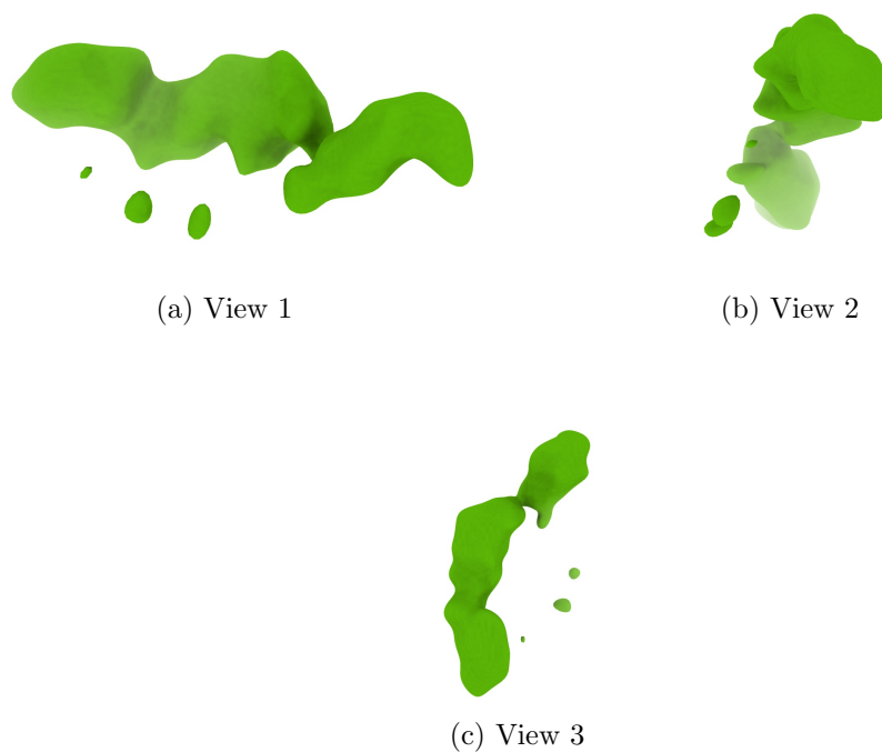
Figure 4: Isosurface at threshold=0.893000. Views generated by ChimeraX at a the following X, Y, Z angles: View 1 (0, -90, -90), View 2 (-90, 0, -90), View 3 (0, 0, 0).
