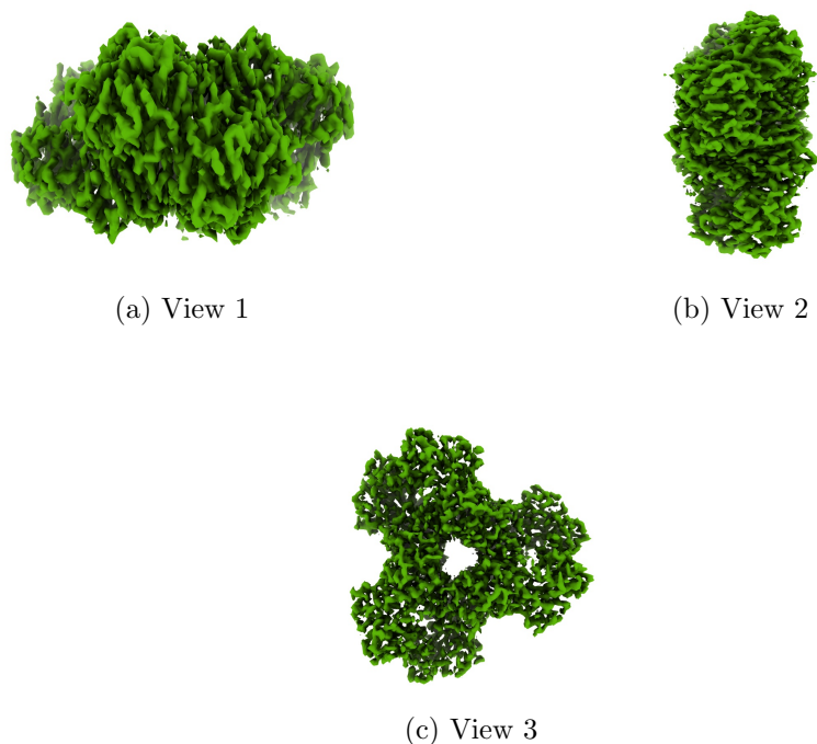
Figure 4: Isosurface at threshold=1.750000. Views generated by ChimeraX at a the following X, Y, Z angles: View 1 (0, -90, -90), View 2 (-90, 0, -90), View 3 (0, 0, 0).
