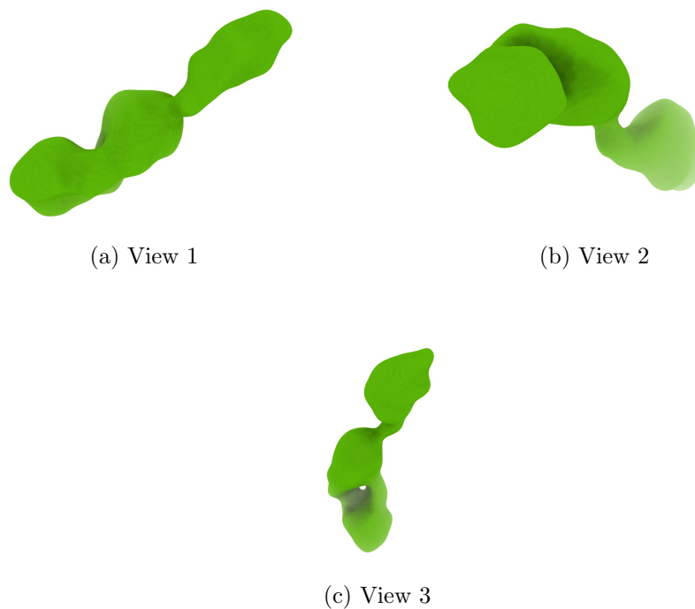
Figure 4: Isosurface at threshold=0.818000. Views generated by ChimeraX at a the following X, Y, Z angles: View 1 (0, -90, -90), View 2 (-90, 0, -90), View 3 (0, 0, 0).
