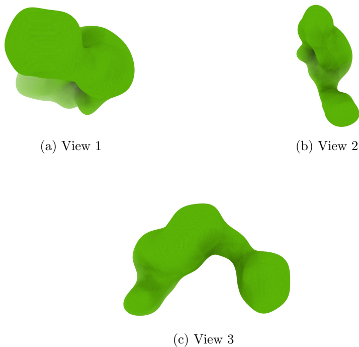
Figure 4: Isosurface at threshold=0.903000. Views generated by ChimeraX at a the following X, Y, Z angles: View 1 (0, -90, -90), View 2 (-90, 0, -90), View 3 (0, 0, 0).
