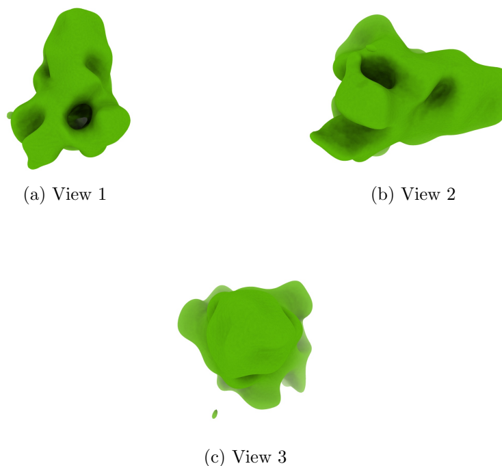
Figure 4: Isosurface at threshold=0.009000. Views generated by ChimeraX at the following X, Y, Z angles: View 1 (0, -90, -90), View 2 (-90, 0, -90), View 3 (0, 0, 0).
