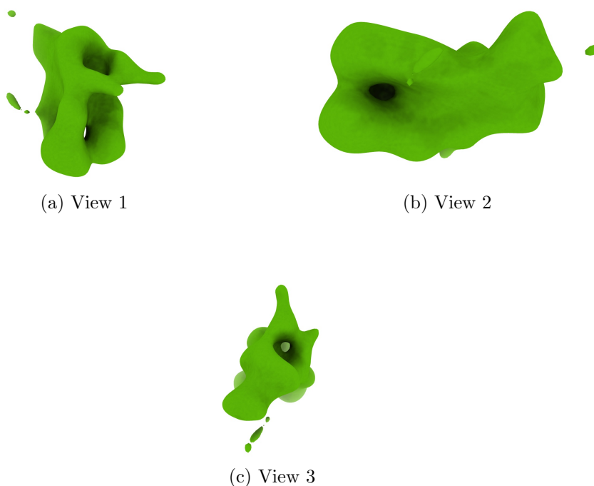
Figure 4: Isosurface at threshold=0.015000. Views generated by ChimeraX at a the following X, Y, Z angles: View 1 (0, -90, -90), View 2 (-90, 0, -90), View 3 (0, 0, 0).
