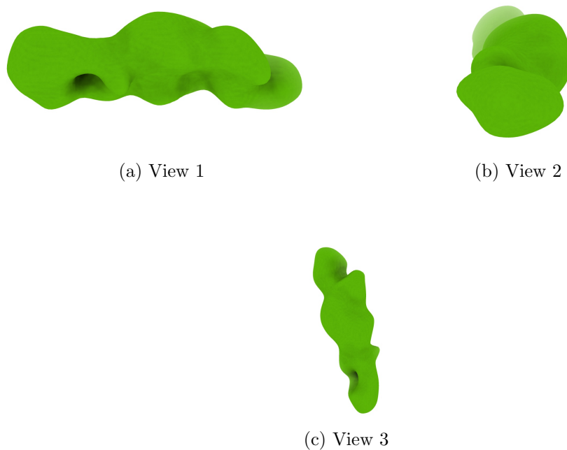
Figure 4: Isosurface at threshold=0.847000. Views generated by ChimeraX at a the following X, Y, Z angles: View 1 (0, -90, -90), View 2 (-90, 0, -90), View 3 (0, 0, 0).
