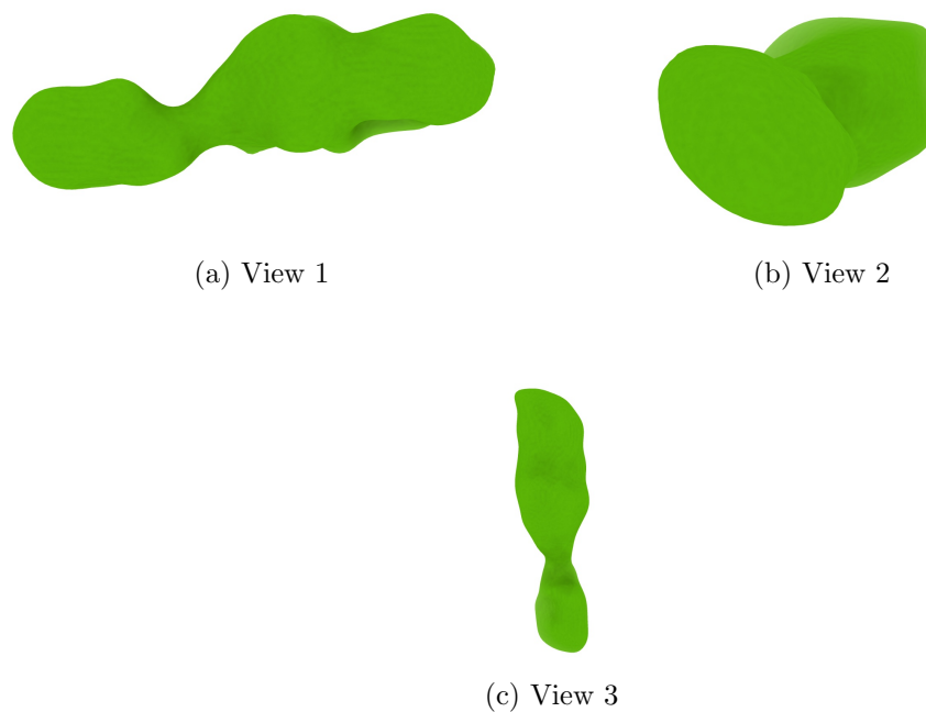
Figure 4: Isosurface at threshold=0.803000. Views generated by ChimeraX at a the following X, Y, Z angles: View 1 (0, -90, -90), View 2 (-90, 0, -90), View 3 (0, 0, 0).
