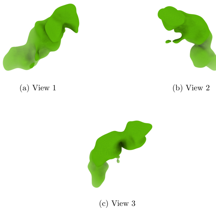
Figure 4: Isosurface at threshold=0.916000. Views generated by ChimeraX at a the following X, Y, Z angles: View 1 (0, -90, -90), View 2 (-90, 0, -90), View 3 (0, 0, 0).
