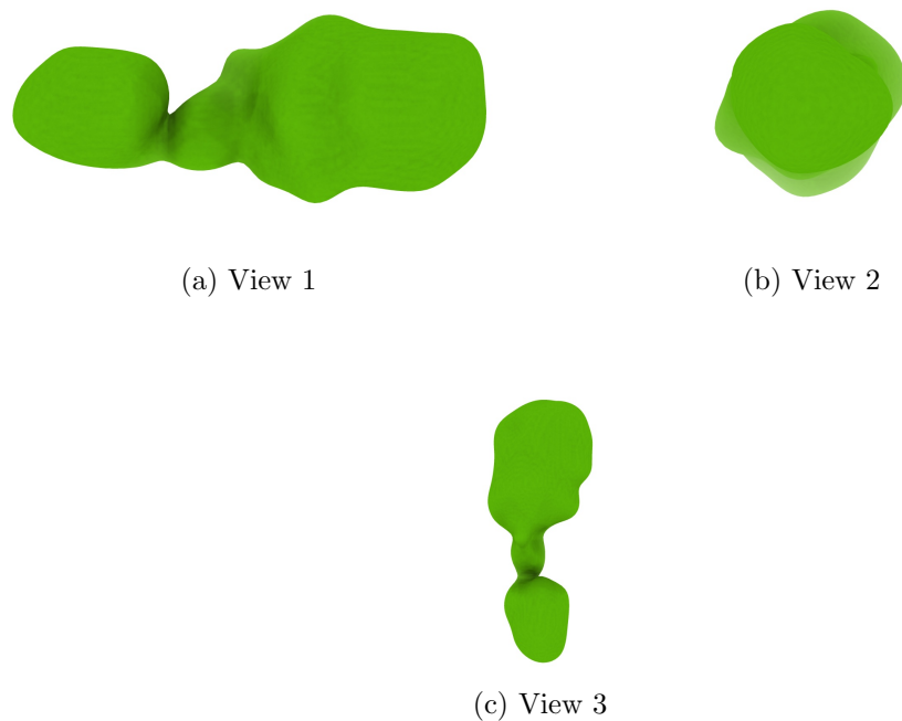
Figure 4: Isosurface at threshold=0.786000. Views generated by ChimeraX at a the following X, Y, Z angles: View 1 (0, -90, -90), View 2 (-90, 0, -90), View 3 (0, 0, 0).
