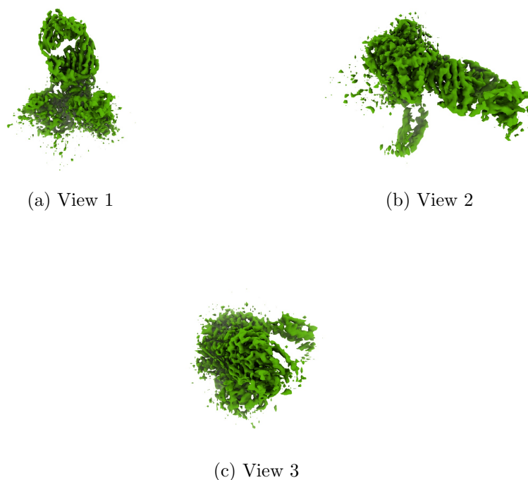
Figure 4: Isosurface at threshold=0.346000. Views generated by ChimeraX at a the following X, Y, Z angles: View 1 (0, -90, -90), View 2 (-90, 0, -90), View 3 (0, 0, 0).
