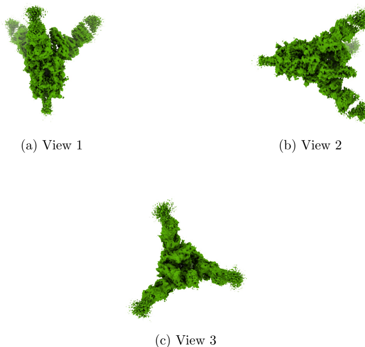
Figure 4: Isosurface at threshold=0.099800. Views generated by ChimeraX at a the following X, Y, Z angles: View 1 (0, -90, -90), View 2 (-90, 0, -90), View 3 (0, 0, 0).
