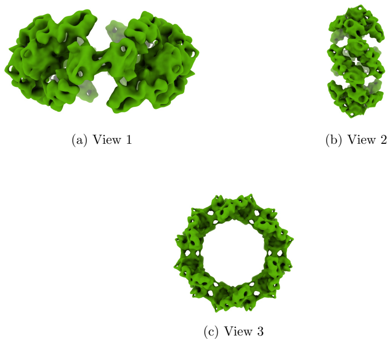
Figure 4: Isosurface at threshold=5.700000. Views generated by ChimeraX at a the following X, Y, Z angles: View 1 (0, -90, -90), View 2 (-90, 0, -90), View 3 (0, 0, 0).
