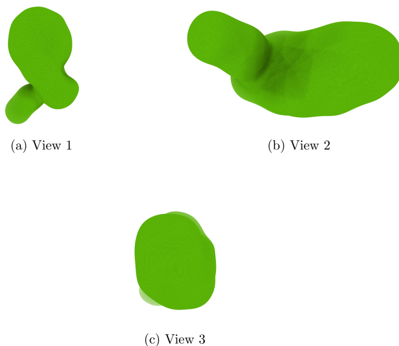
Figure 4: Isosurface at threshold=1.700000. Views generated by ChimeraX at a the following X, Y, Z angles: View 1 (0, -90, -90), View 2 (-90, 0, -90), View 3 (0, 0, 0).
