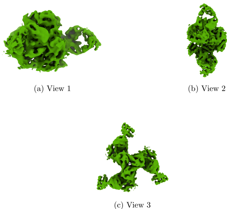
Figure 4: Isosurface at threshold=1.020000. Views generated by ChimeraX at a the following X, Y, Z angles: View 1 (0, -90, -90), View 2 (-90, 0, -90), View 3 (0, 0, 0).
