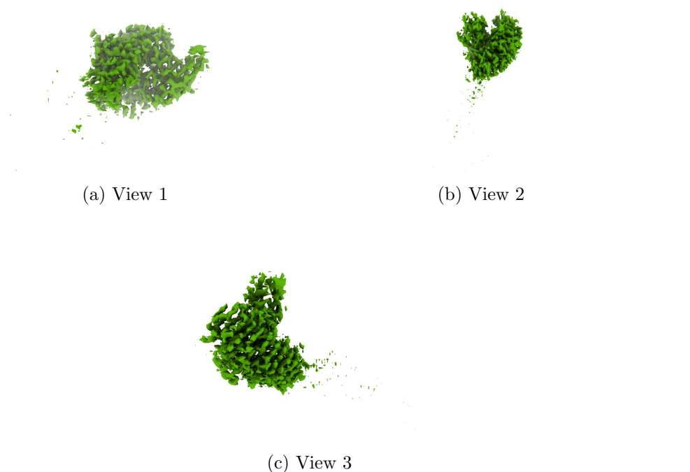
Figure 4: Isosurface at threshold=0.719000. Views generated by ChimeraX at a the following X, Y, Z angles: View 1 (0, -90, -90), View 2 (-90, 0, -90), View 3 (0, 0, 0).
