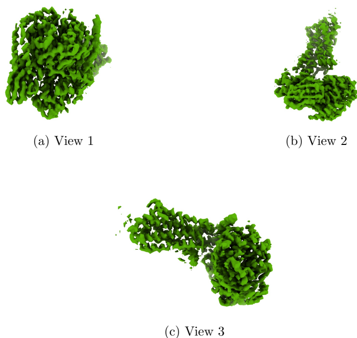
Figure 4: Isosurface at threshold=0.396000. Views generated by ChimeraX at a the following X, Y, Z angles: View 1 (0, -90, -90), View 2 (-90, 0, -90), View 3 (0, 0, 0).
