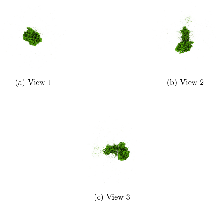
Figure 4: Isosurface at threshold=0.177000. Views generated by ChimeraX at a the following X, Y, Z angles: View 1 (0, -90, -90), View 2 (-90, 0, -90), View 3 (0, 0, 0).
