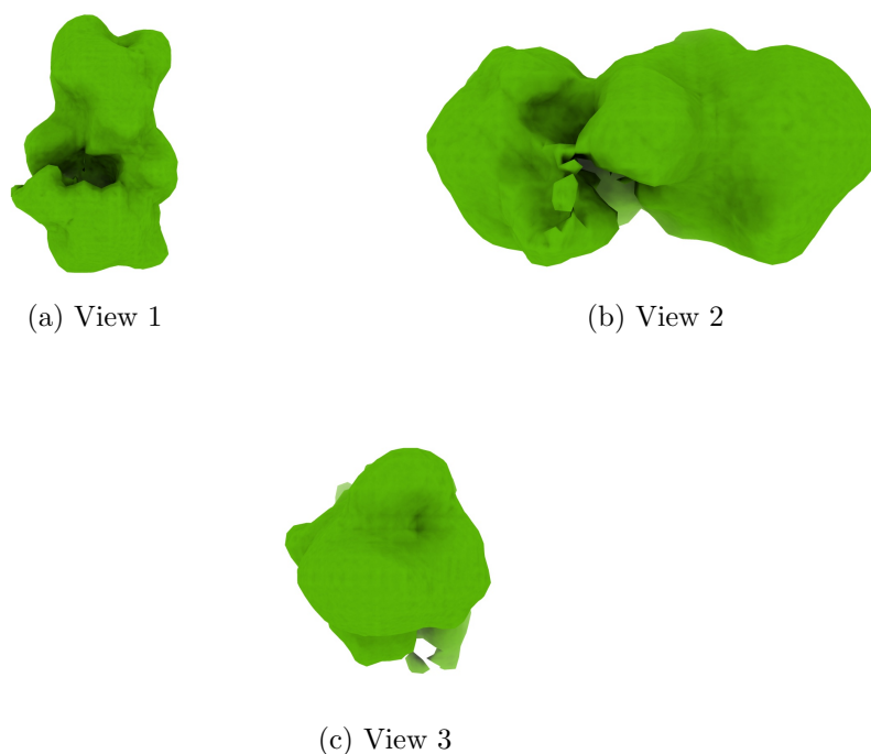
Figure 4: Isosurface at threshold=4.420000. Views generated by ChimeraX at a the following X, Y, Z angles: View 1 (0, -90, -90), View 2 (-90, 0, -90), View 3 (0, 0, 0).
