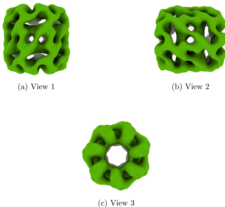
Figure 4: Isosurface at threshold=0.173000. Views generated by ChimeraX at a the following X, Y, Z angles: View 1 (0, -90, -90), View 2 (-90, 0, -90), View 3 (0, 0, 0).
