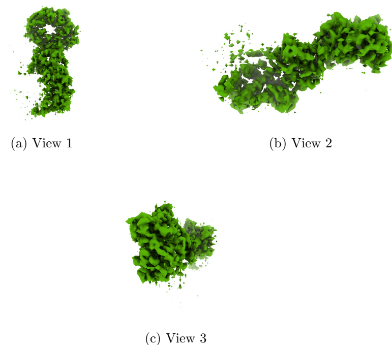
Figure 4: Isosurface at threshold=0.264000. Views generated by ChimeraX at a the following X, Y, Z angles: View 1 (0, -90, -90), View 2 (-90, 0, -90), View 3 (0, 0, 0).
